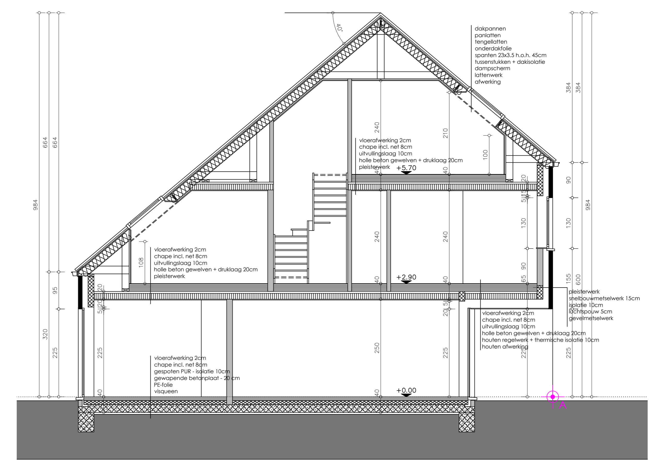
Doorsnede 2-2 (lot 73)
