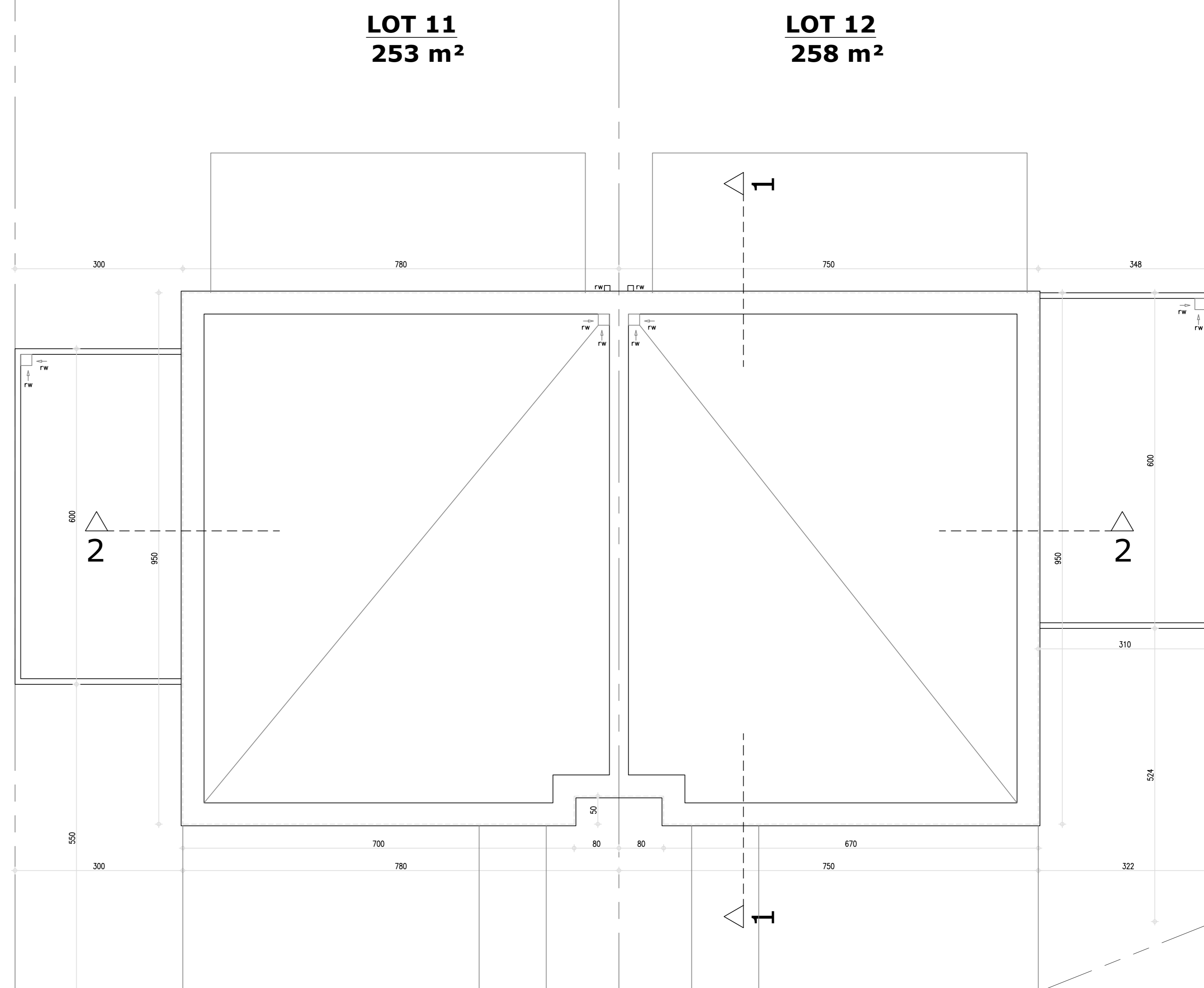
DAKENPLAN 1/50
