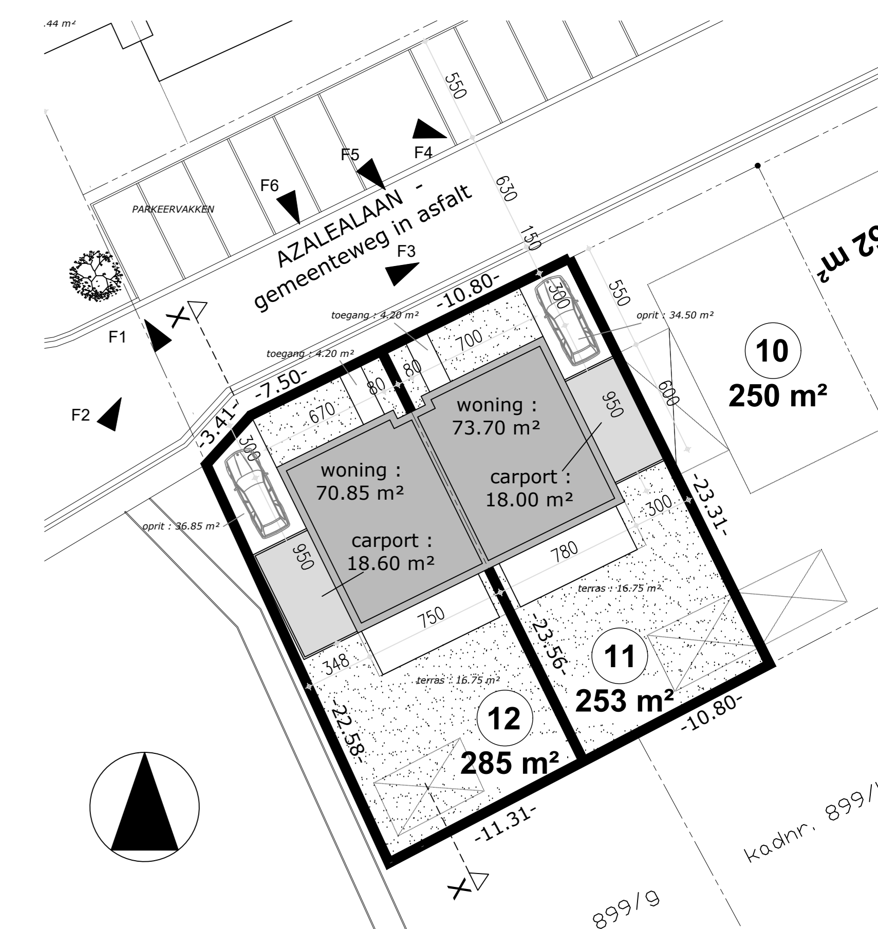
INPLANTINGSPLAN 1/200
