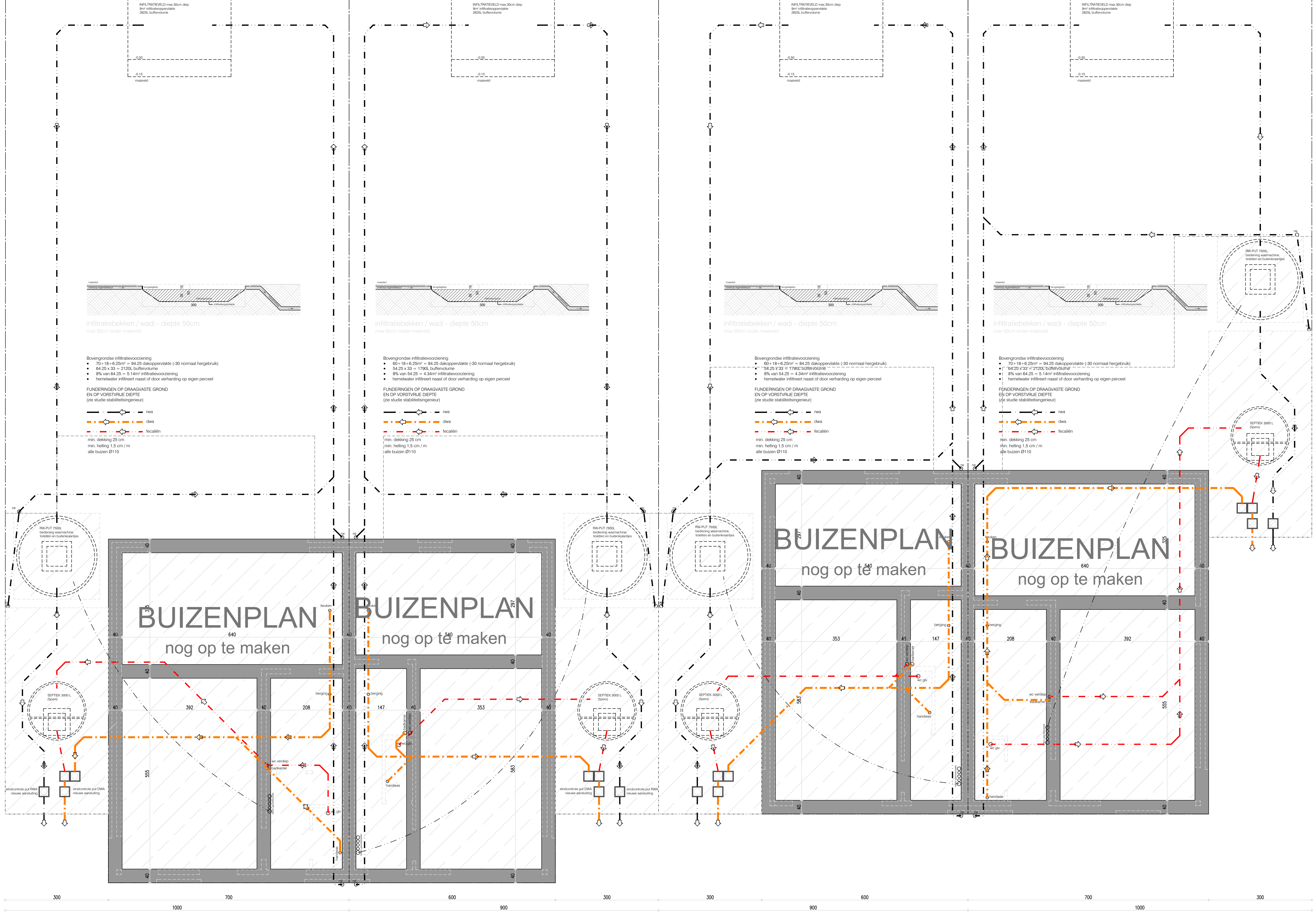
funderings- en rioleringsplan lot 11 70.00 m 2 bruto opp. funderings- en rioleringsplan lot 10 60.00 m 2 bruto opp. funderings- en rioleringsplan lot 9 60.00 m 2 bruto opp. funderings- en rioleringsplan lot 8 70.00 m 2 bruto opp.
