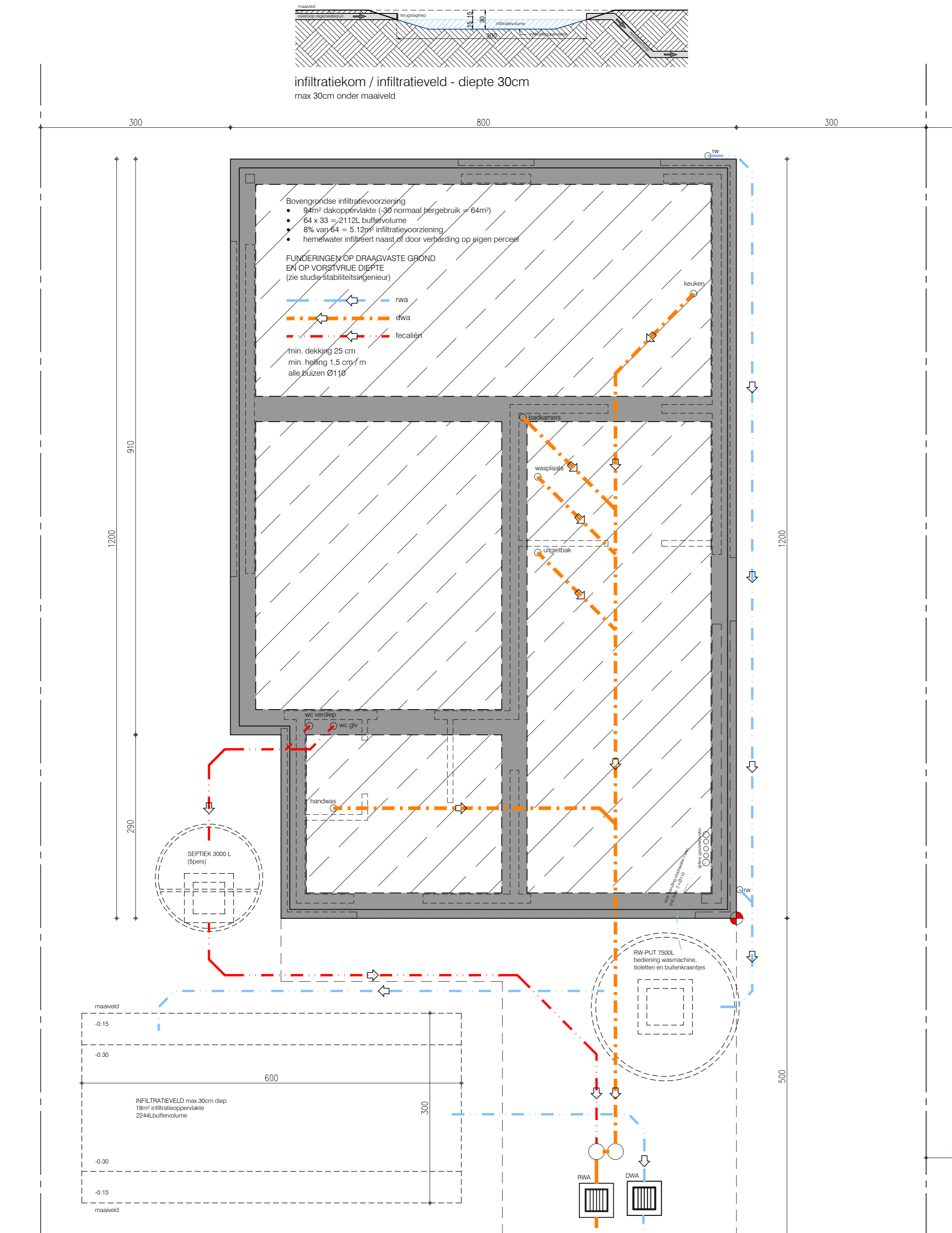
riolerings- en funderingsplan lot 78 93.68 m 2 bruto opp.
