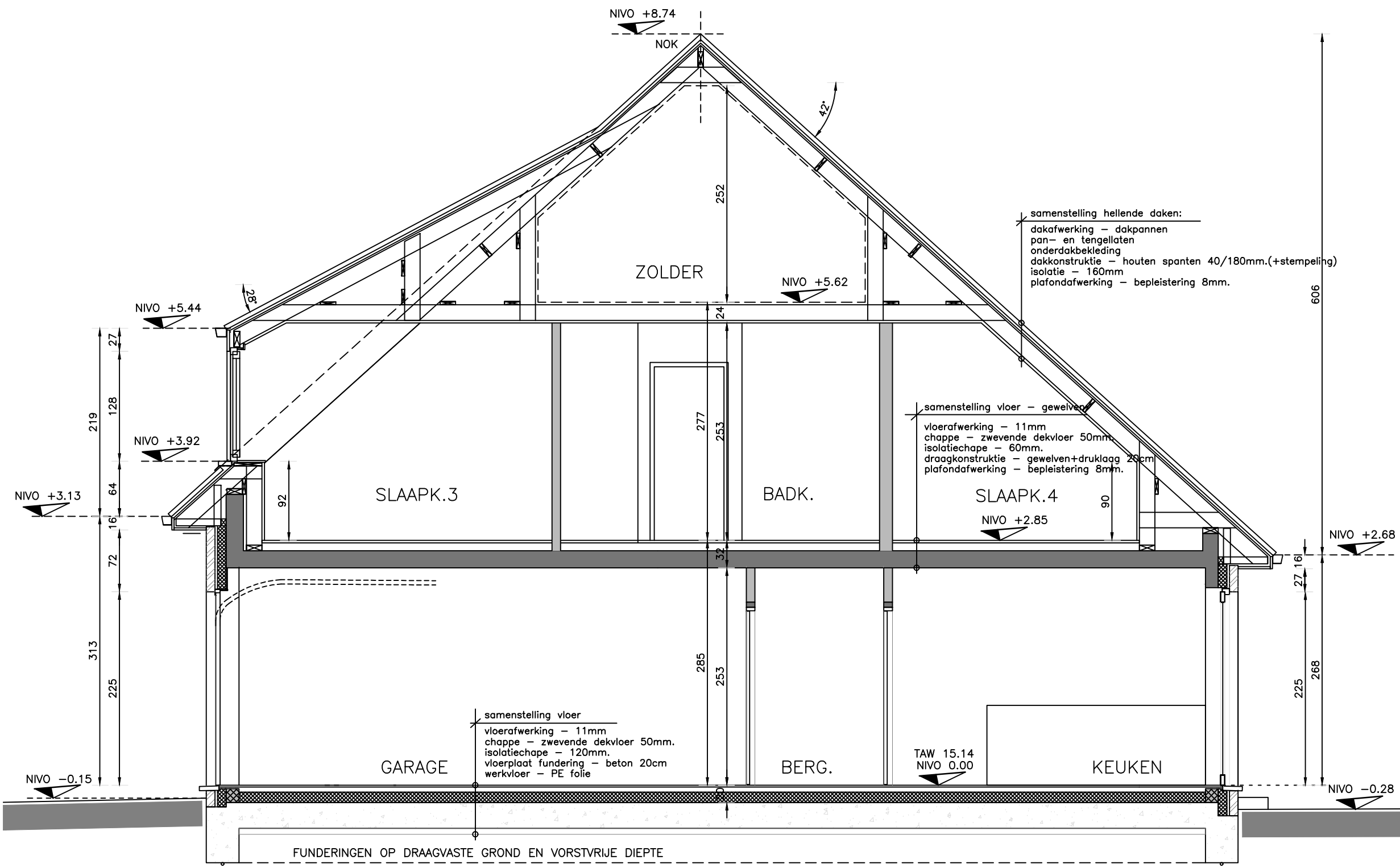
Doorsnede H-H Lot 15
