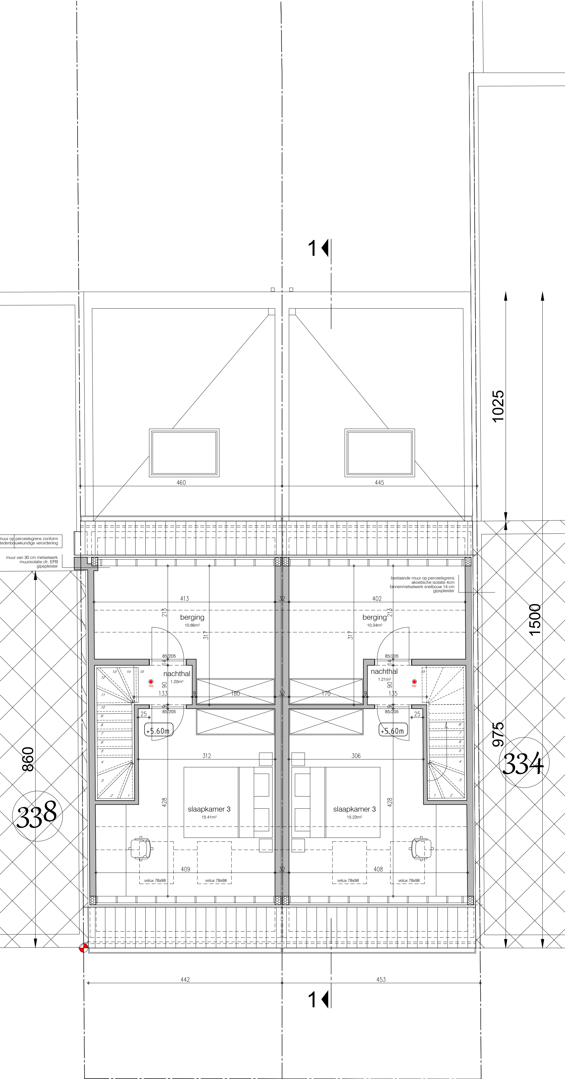
dakverdieping lot 1
