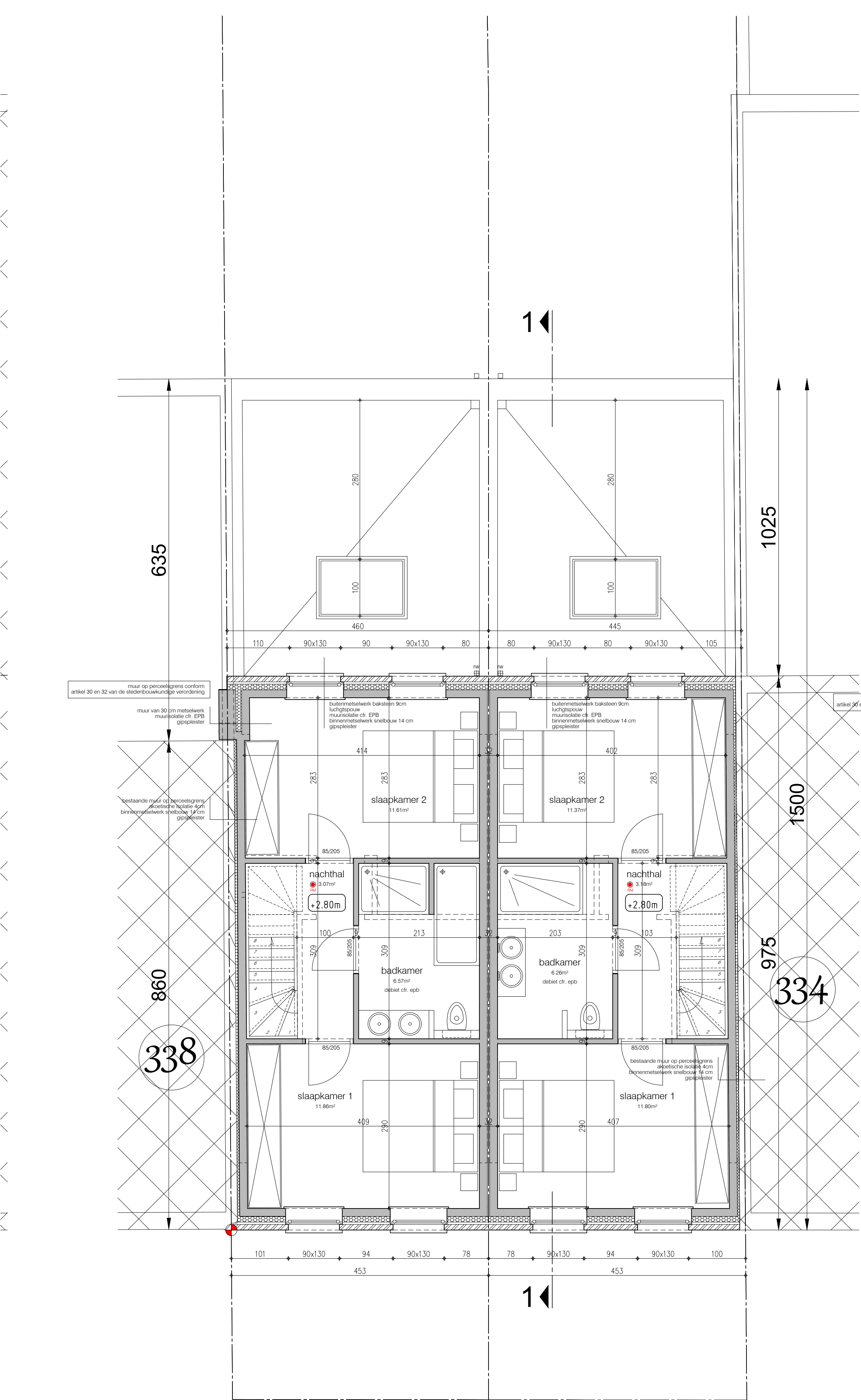
1ste verdieping lot 1
