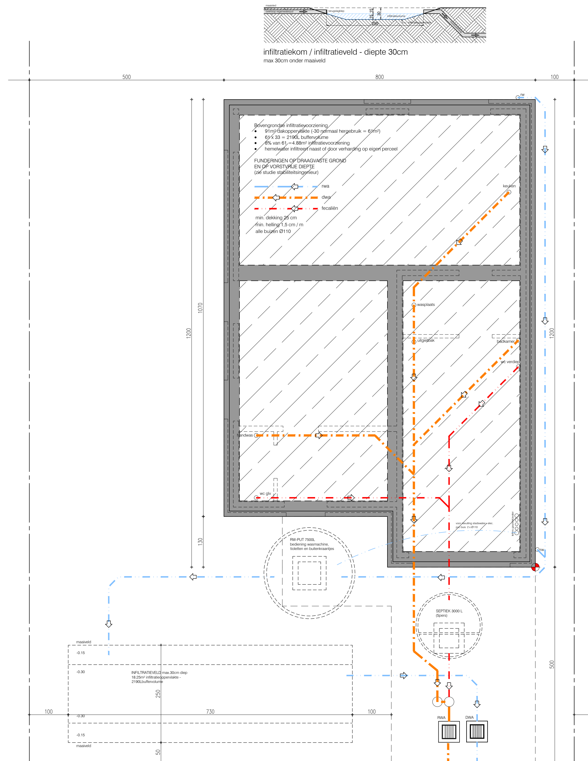
riolerings- en funderingsplan lot 77 90.54 m 2 bruto opp.
