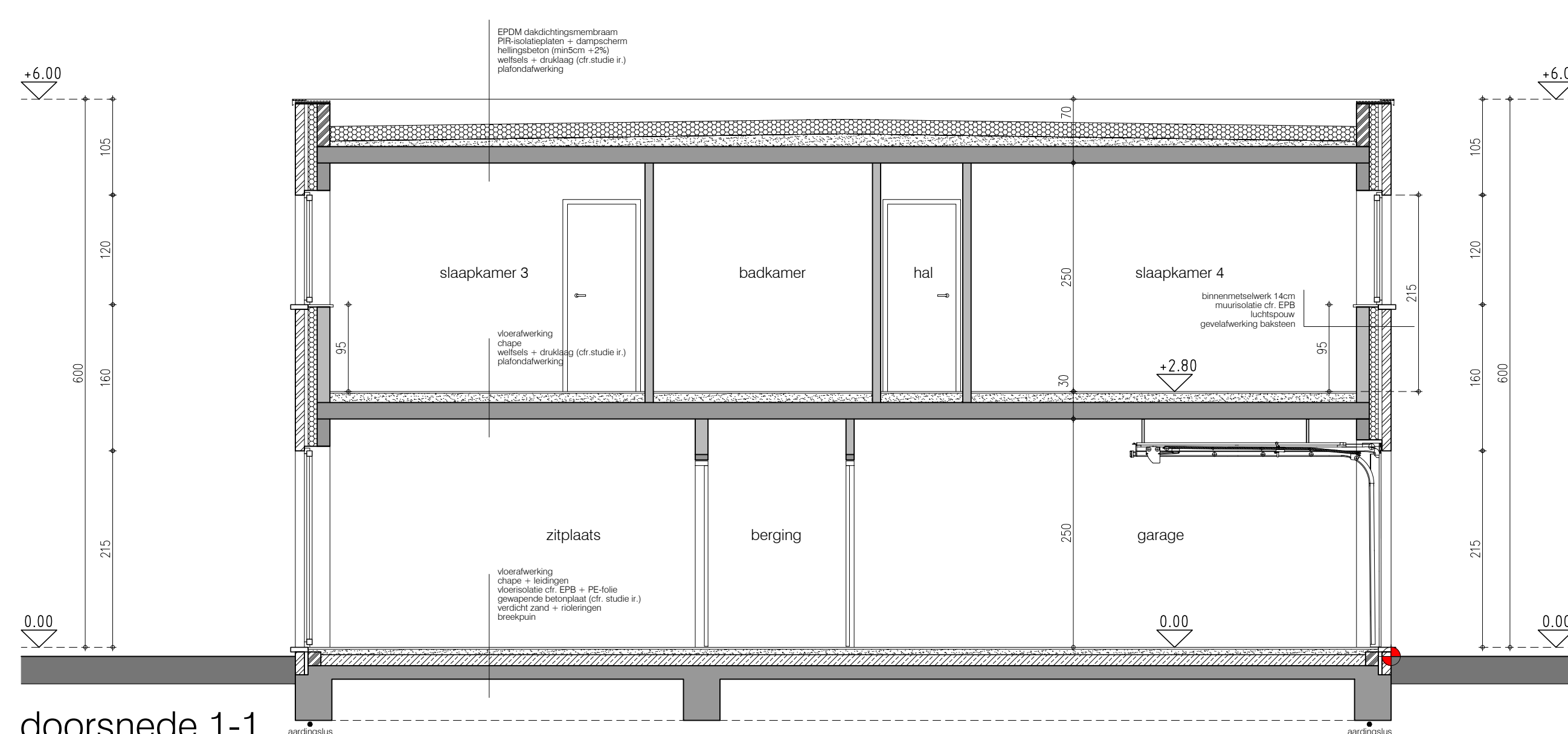
doorsnede 1-1 lot 77
